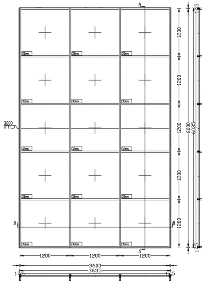
Figure 1 Sketch of the representative product for the curtain wall
