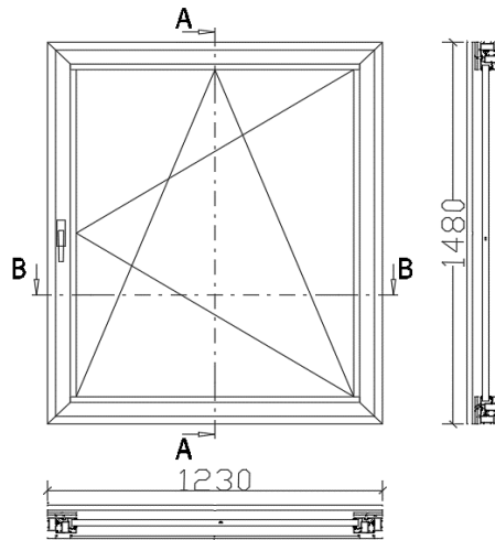
Figure 1 Sketch of the representative product for the hinged non-insulated system
