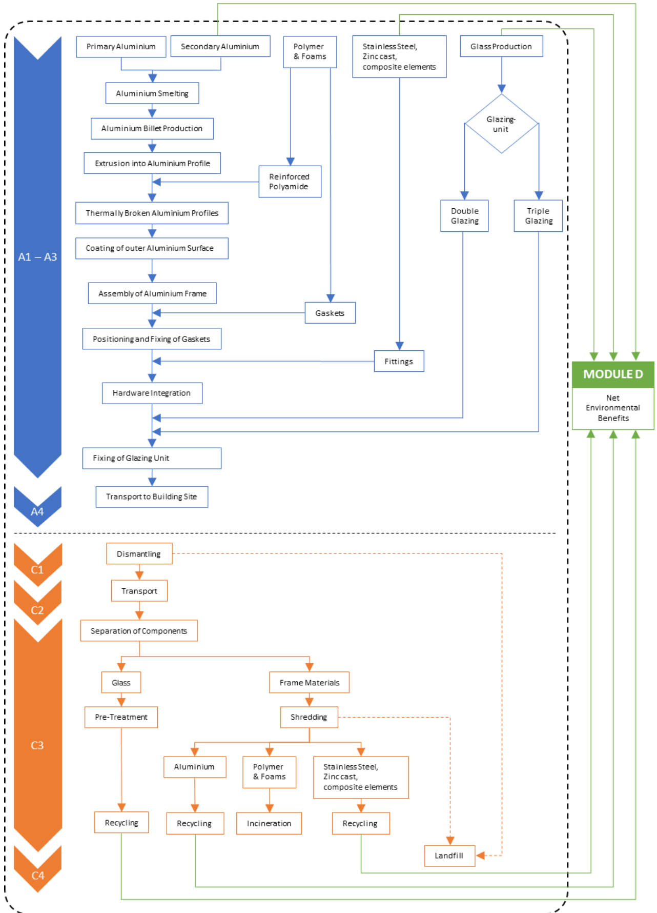
Figure 2 Main production processes and components of the hinged non-insulated system
