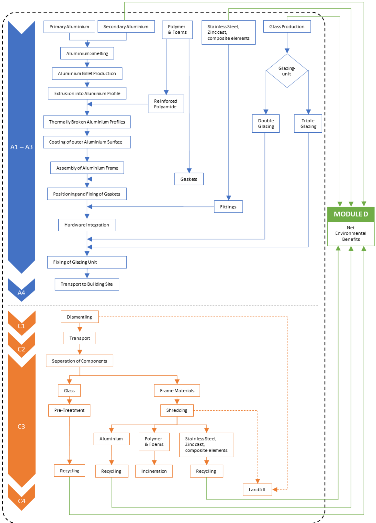
Figure 2 Main production processes and components of the sliding insulated system
