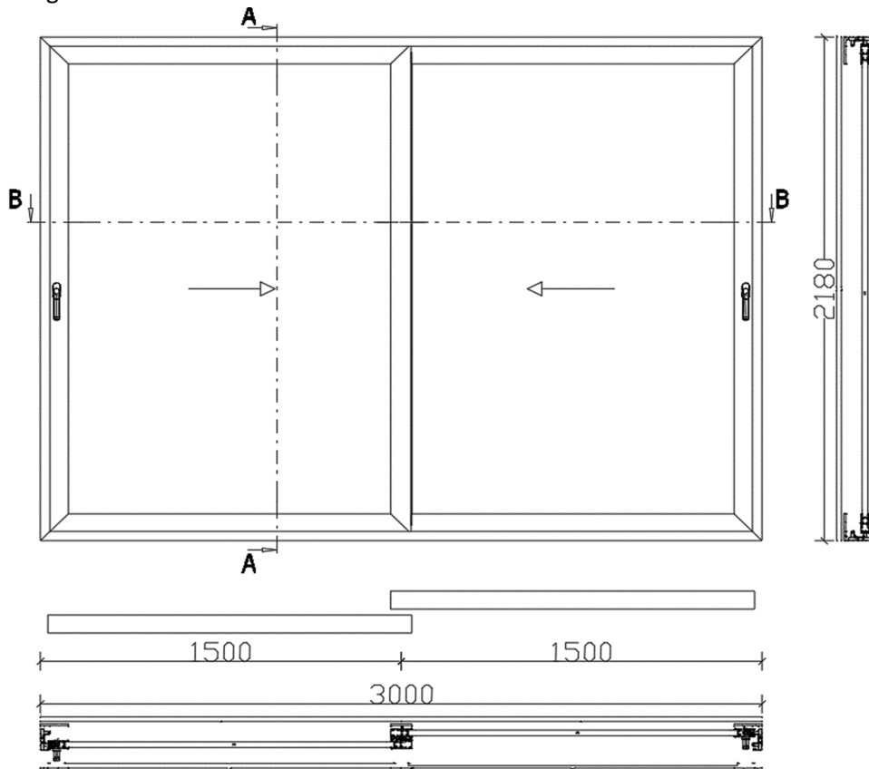
Figure 1 Sketch of the representative product for the sliding insulated system
