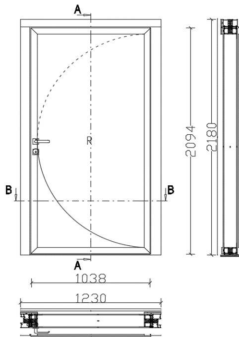
Figure 1 Sketch of the representative product for the entrance doors insulated system
