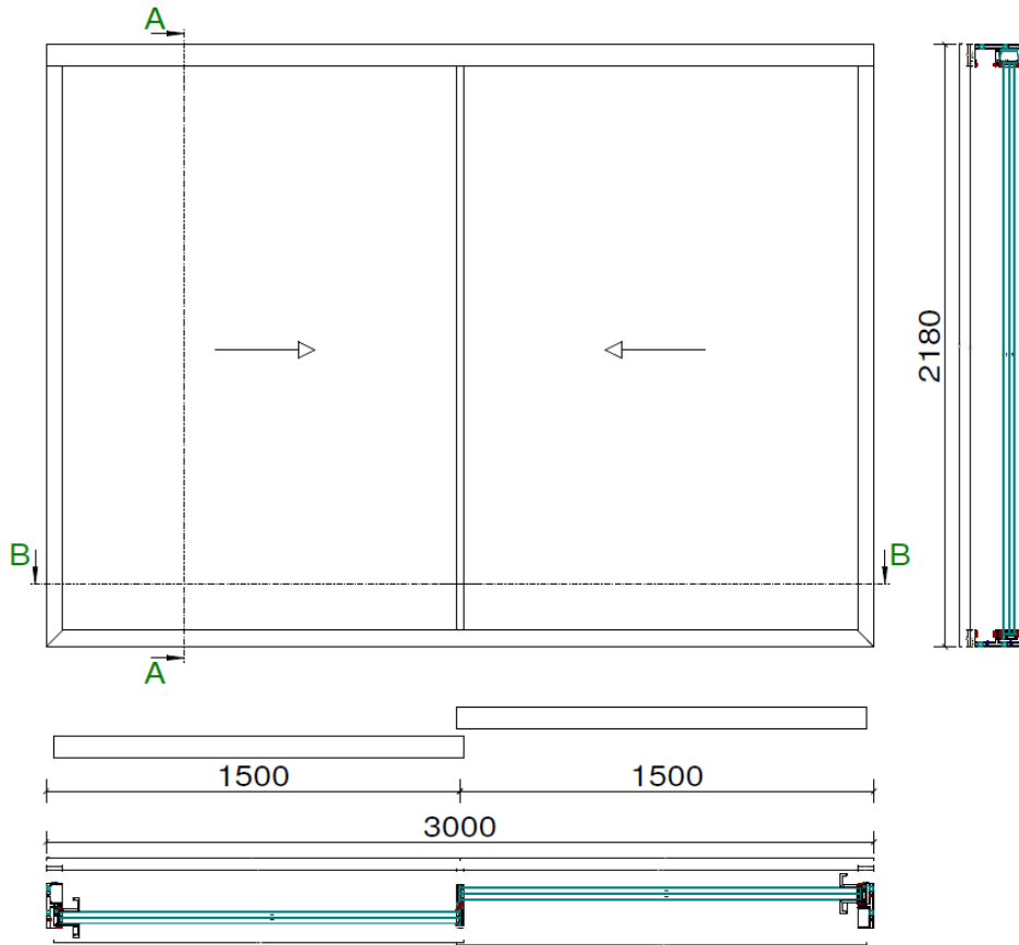
Figure 1. Sketch of the representative product for the S650 sliding door (size in mm)
