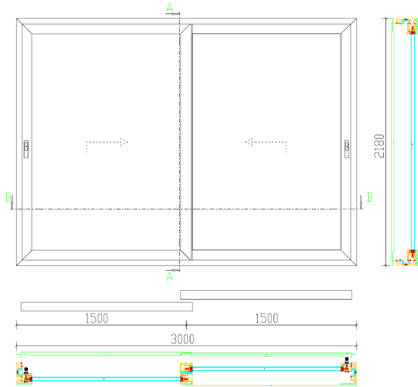
Figure 1. Sketch of the representative product for the S700 sliding door (size in mm)
